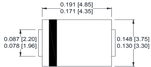
SMB/ DO-214AA
