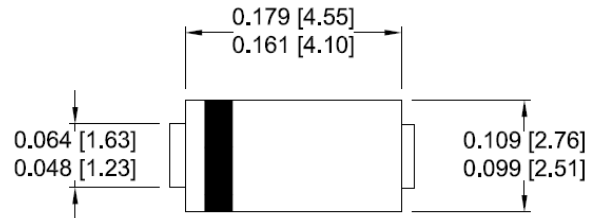
SMA/ DO-214AC
